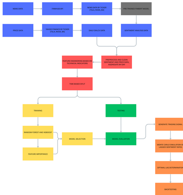
End-to-End Sentiment-Driven Trading Pipeline
